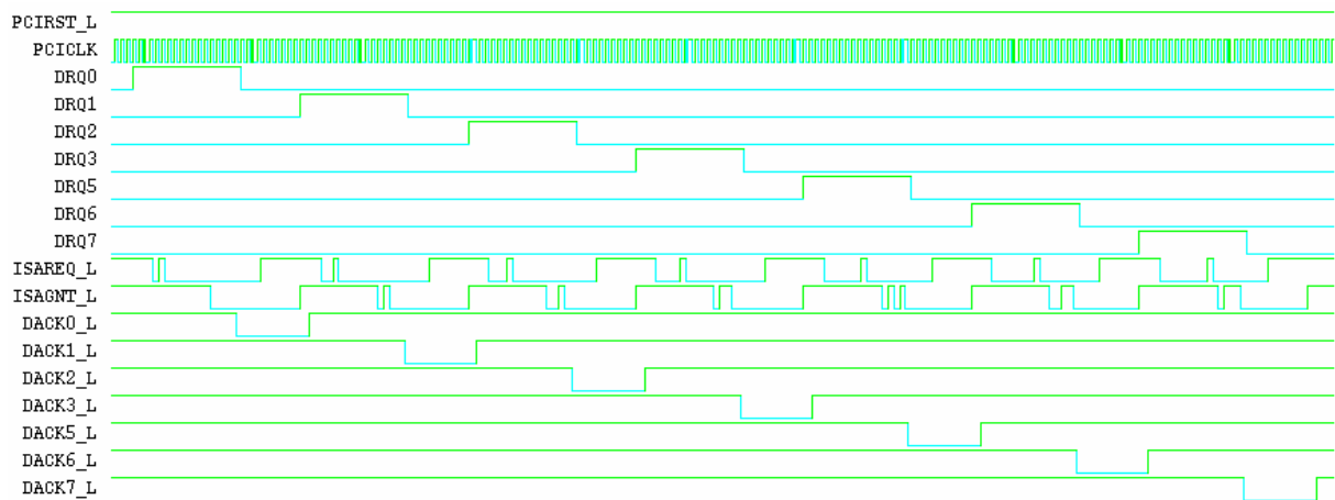
Figure 13-18: DRQn/DACKn# Coding in PC/PCI DMA Function
