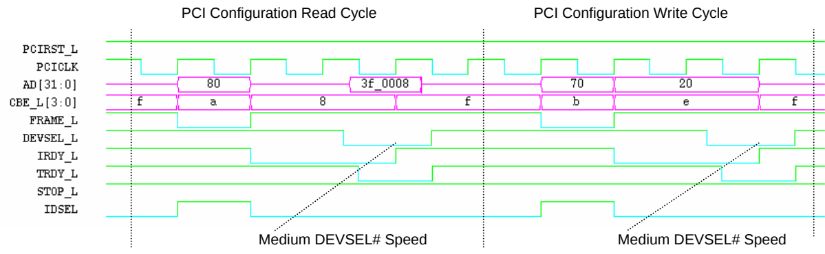
Figure 13-5: PCI Configuration Read/Write Cycle
